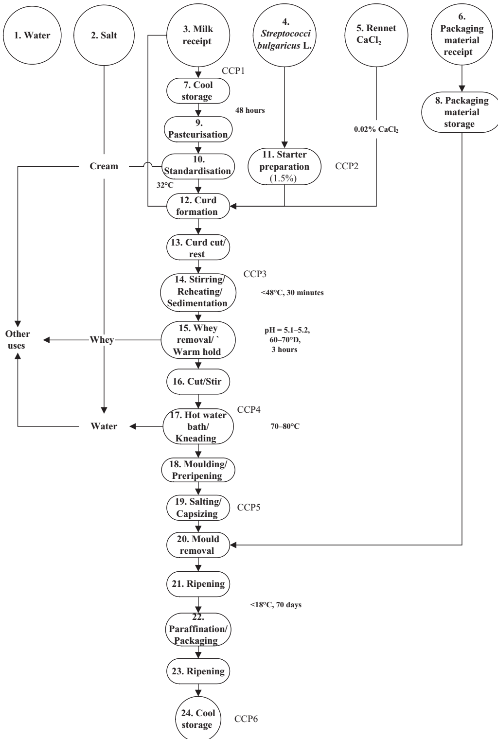
Fig. 3.3 Kasserri/semi-hard cheese flow diagram.
