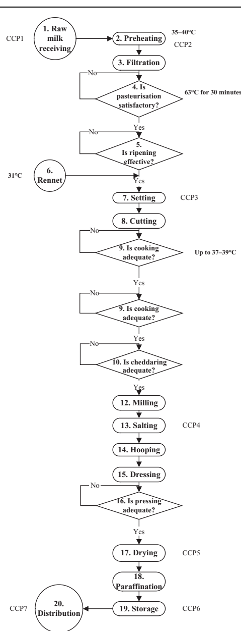
Fig. 3.8 Cheddar cheese manufacturing flow diagram.
