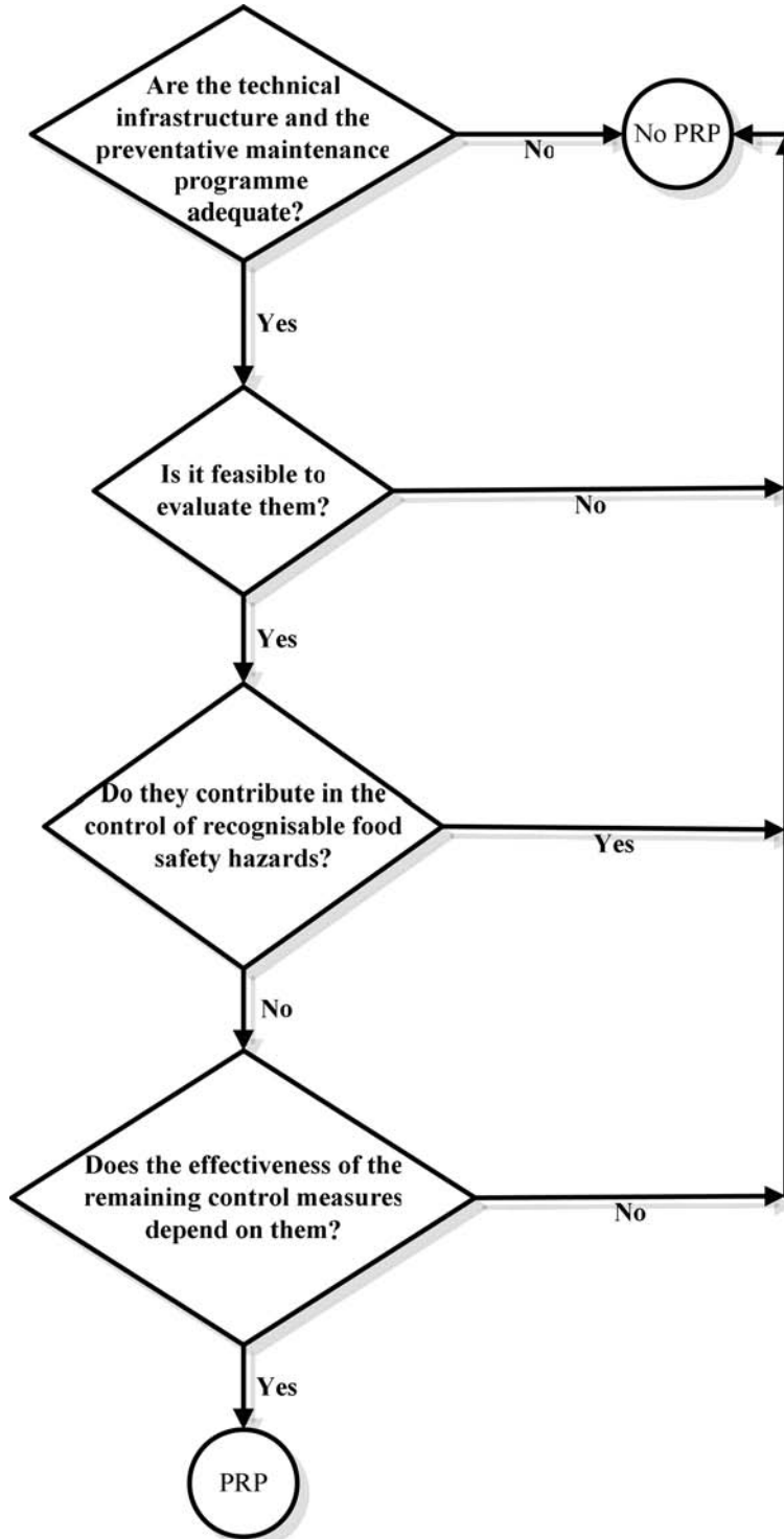
Fig. 1.13 Tree diagram for determination of prerequisite programmes according to ISO 22000.
