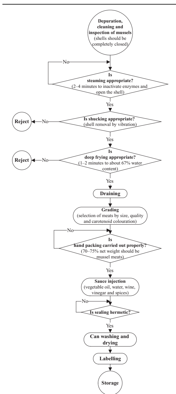
Fig. 7.7 Flow diagram for production of canned pickled mussels.
