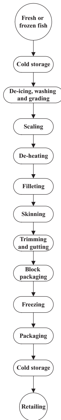
Fig. 7.2 Flow diagram for filleting of white and oily fish.
