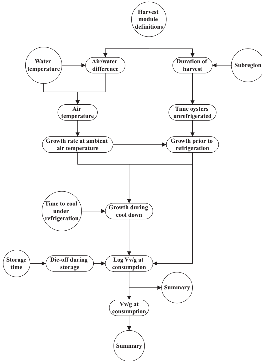
Fig. 7.3 Structure of simulation model of effect of post-harvest handling on Vibrio vulnificus/g (Vv/g) density.
